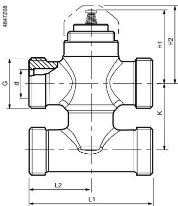
3-port valves with bypass VMP47..
