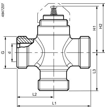
3-port valves VXP47..
