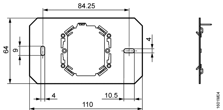
Base plate rectangular
