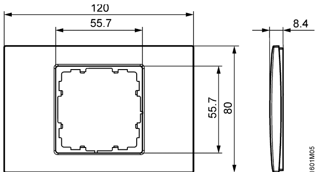
Bezel similar to DELTA azio (rectangular)
