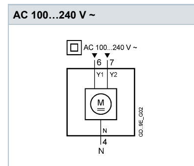
GDB341.9E (open-close, three-p.)
