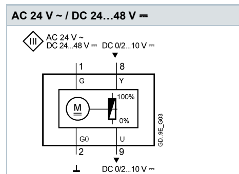
GDB161.9E (modulating)
