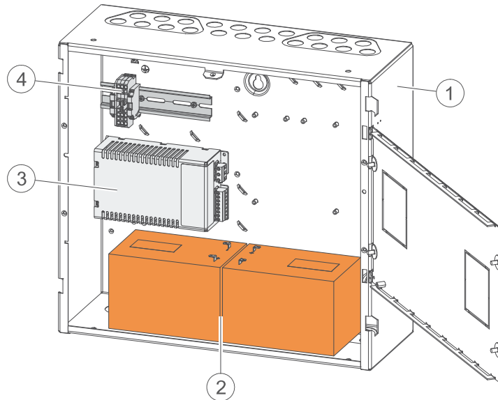
Fig. 1: Arranging the components, using the housing (Standard) as an example
