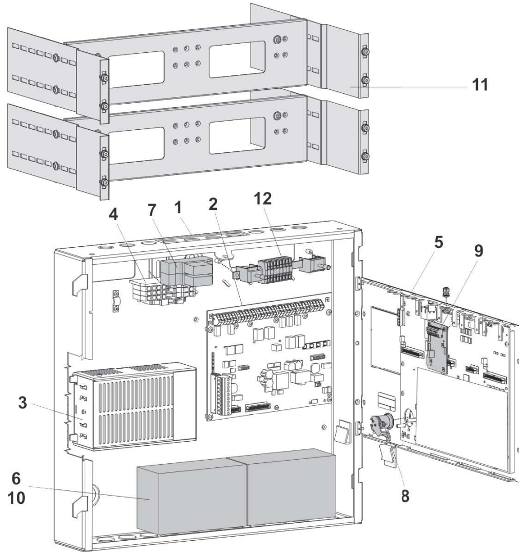
Fig. 2: Layout of FC721
