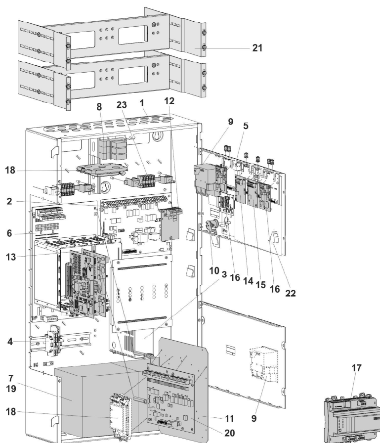
Fig. 4: Layout of FC723
