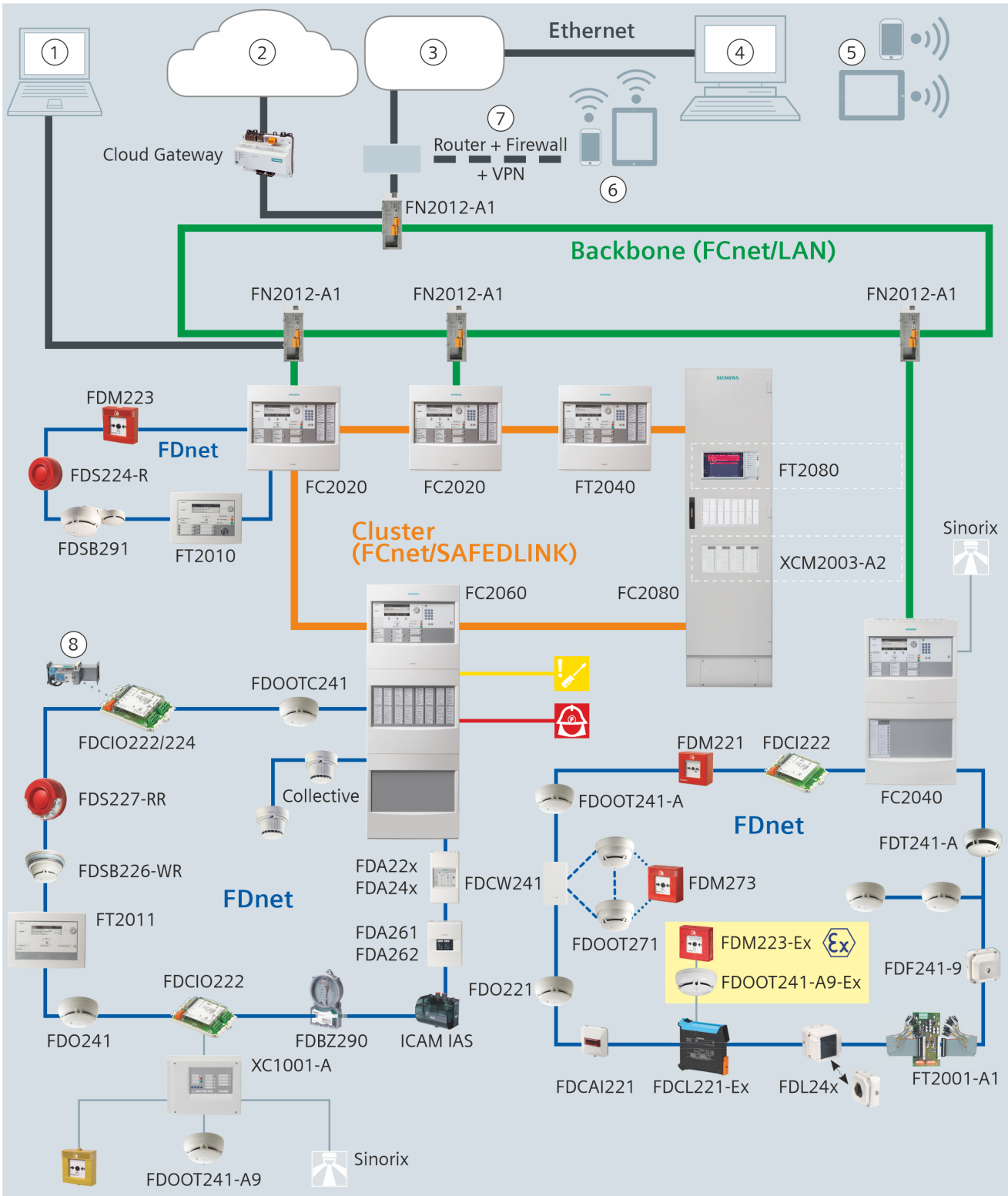
Fig. 1: System overview
